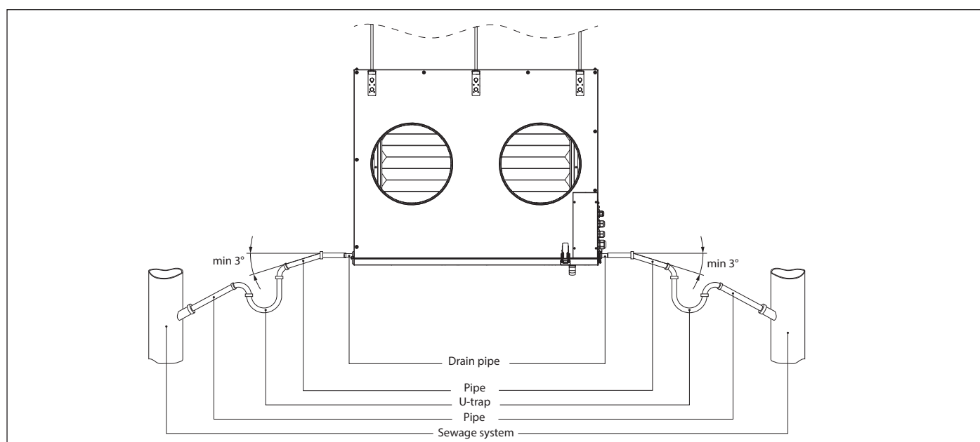
Fig. 8. Condensate drainage
