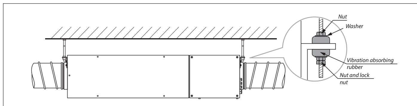
Fig. 7. Mounting
