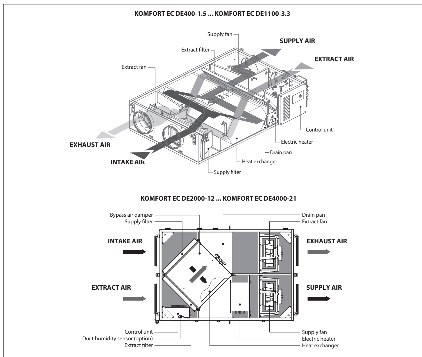
Fig. 1. Unit design and operating logic
