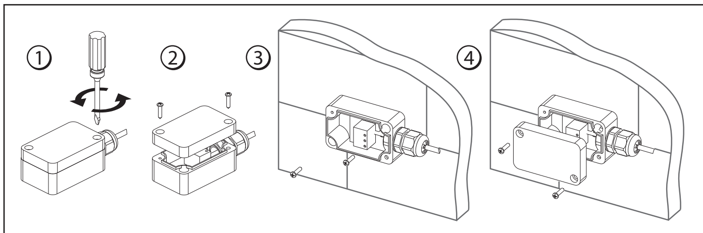
Fig. 13. Outdoor temperature sensor mounting
