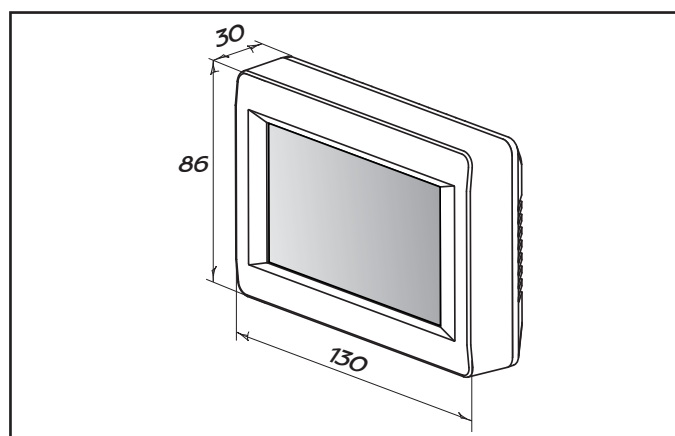
Fig. 14. Control panel overall dimensions
