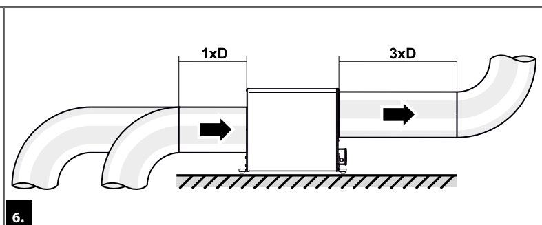
General mounting recommendations for Iso-ZS fans
