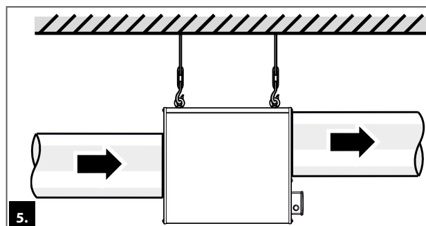
Iso-ZS fan mounting and operation example
