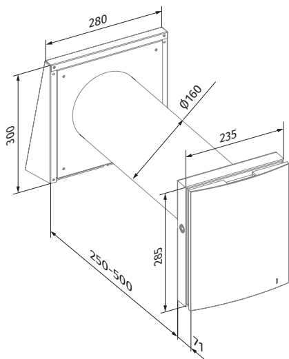
Vento Expert A50C3-1 S8 W V.2
