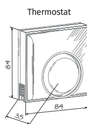
Thermostat
