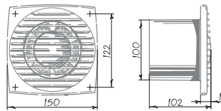
Ventilator Bravo Still 100
