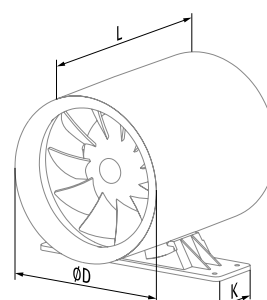
Ducto-U
